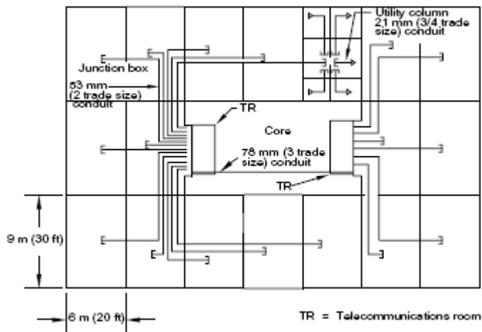
Figure 4.29: Typical zoned ceiling (plan view)
